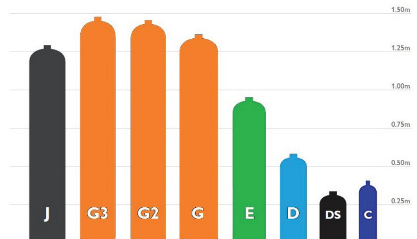
High Pressure Aluminium Cylinders - GASGRAB colour code reference
